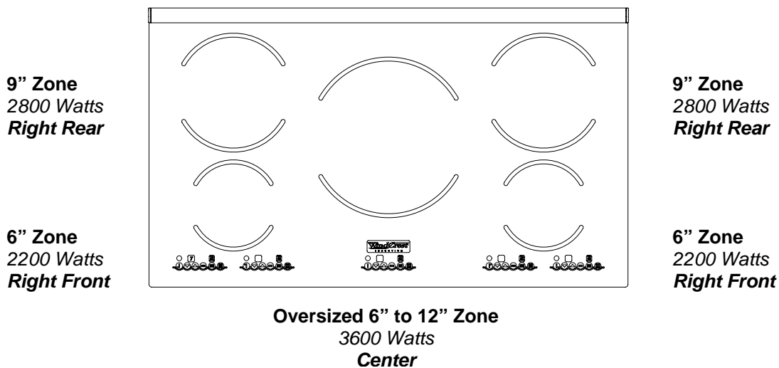
CTI365D (top down view) – 36" Induction Cooktop Zone Size and Power
